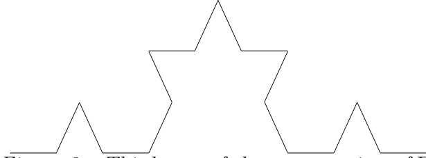
Figure 3 : Third step of the construction of \Gamma .
