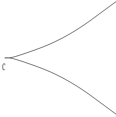
Figure 1 : An example of a domain containing a cusp in \mathbb{C} .
