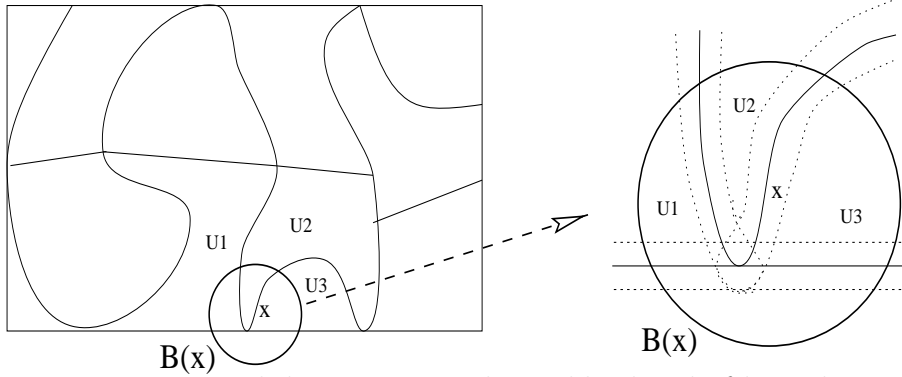
Figure 2 : Typical domains U_i with neighborhood of boundaries.
